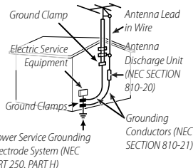
EXAMPLE OF ANTENNA GROUNDING AS PER NATIONAL ELECTRICAL CODE
