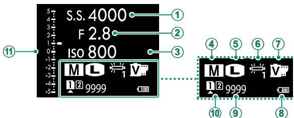
Secundaire LCD-monitor
